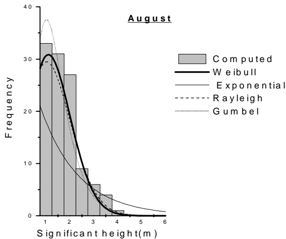
Figure 1. Visually estimated and theoretical significant wave height distribution off Goa.
